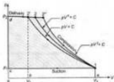
Three types of compression processes on a p-V diagram
