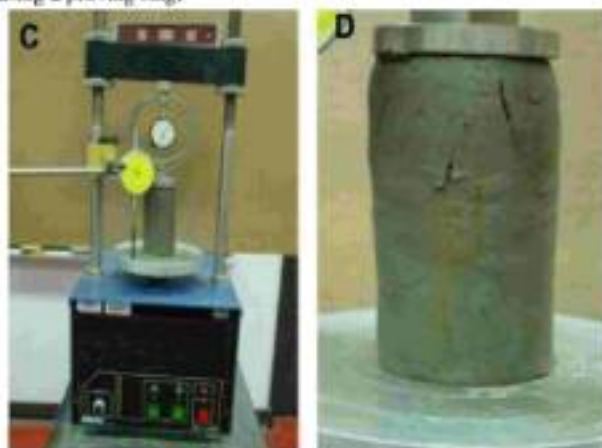
Fig. Unconfined Compressive Strength Test
