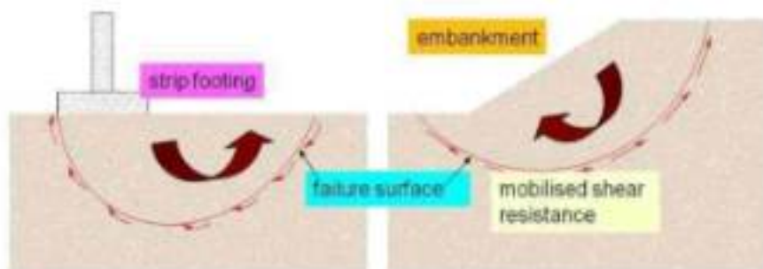
Fig. Shear Failure
