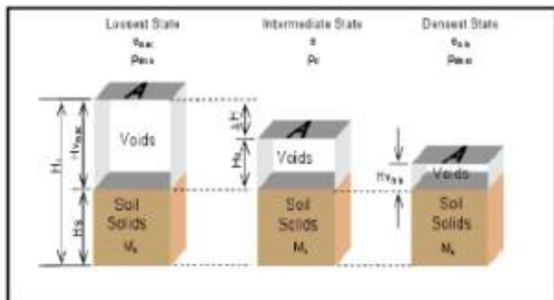
Fig: Volume reduction from compaction of granular soil
