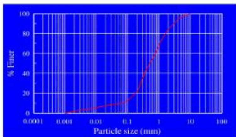
Fig: Particle size distribution graph
