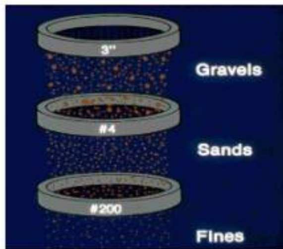
Fig: Set of IS Sieves
