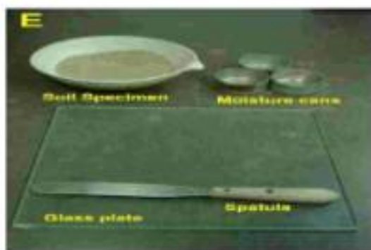
Fig: Shows Plastic limit test apparatus
