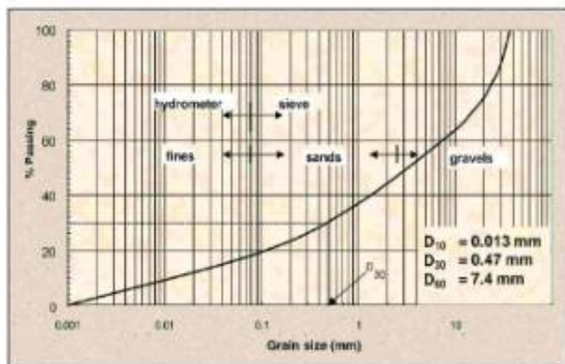
Fig: Illustrates Particle Size Distribution Curve
