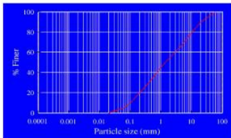
Fig: Grading curves of Well graded soil
