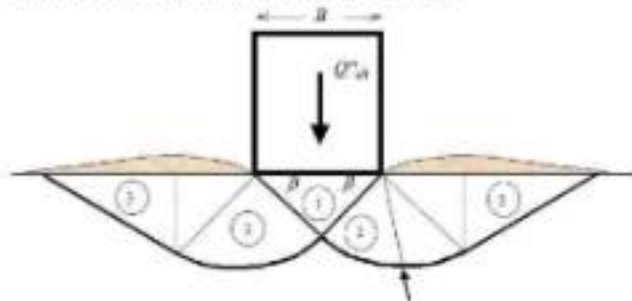
Fig: Shear Failure under Foundation Load
