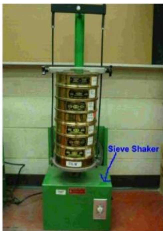
Fig: Illustrates Sieve Analysis test procedure
