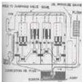
Forced feed Lubrication system
